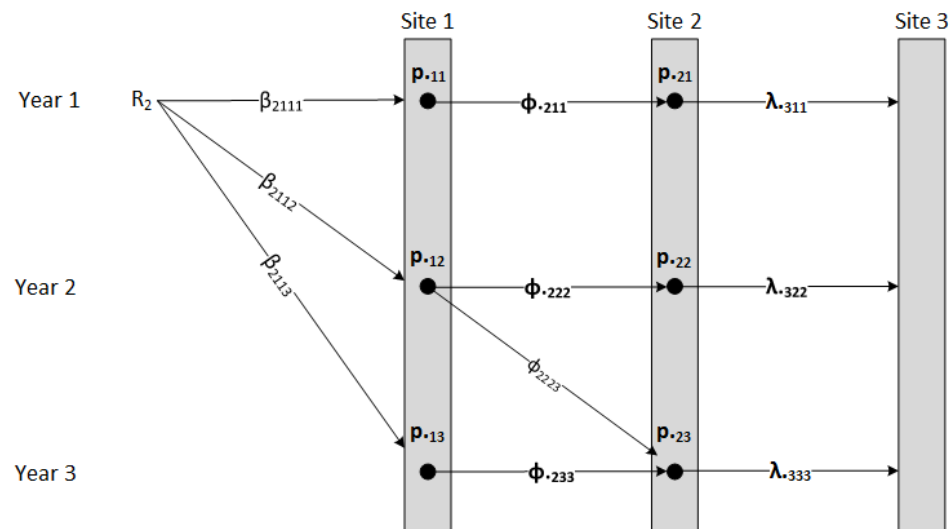
Figure 3. A graphical representation of Model M.y.s.5 with all parameters equated across release sites. The equated parameters are in bold.
